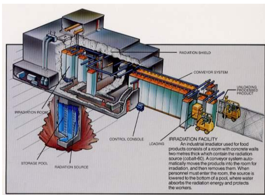
Figure 13: Illustration of an Irradiation Chamber using Cobalt-60 45
